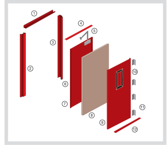
Exploded View
